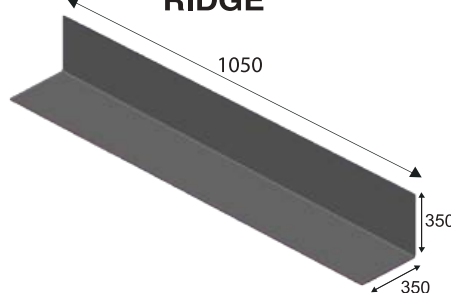
TWR - HYBRID THREE WAY RIDGE
