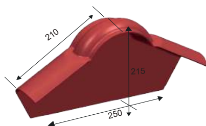
TRC - MAXI TOP RIDGE COVER
