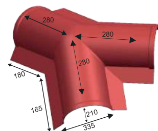
TWR - HYBRID THREE WAY RIDGE
